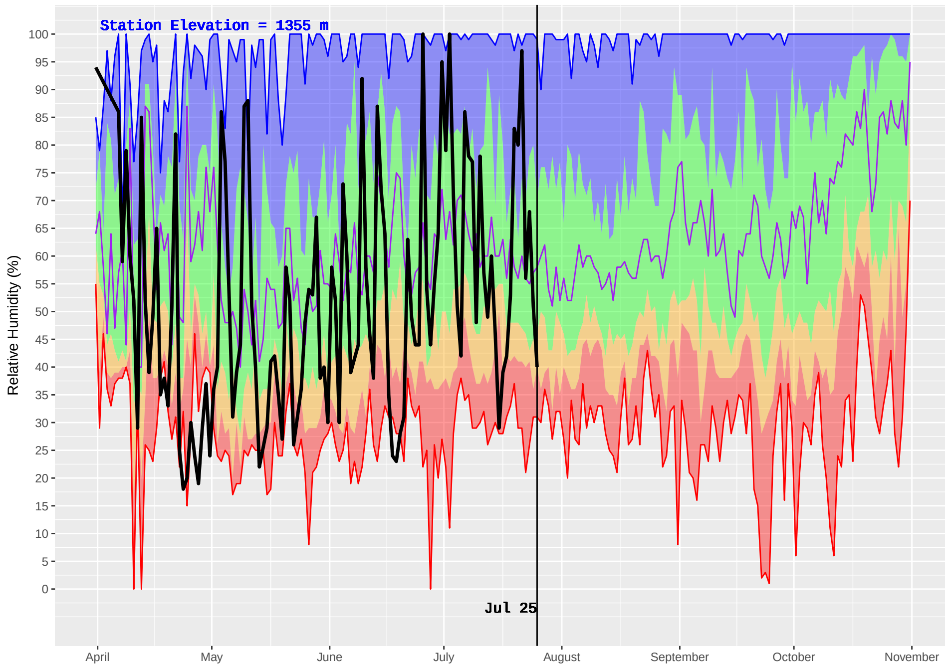
BIG VALLEY (262) : Historical (1987–2016) and Current (2018) Noon Relative Humidity
